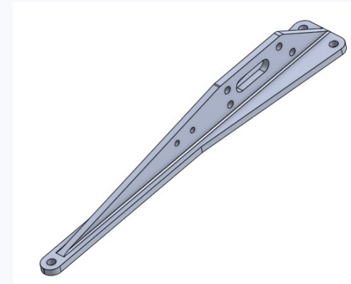
Firewall engine mount bracket / CAD
