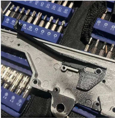
Airsoft tappet plate
